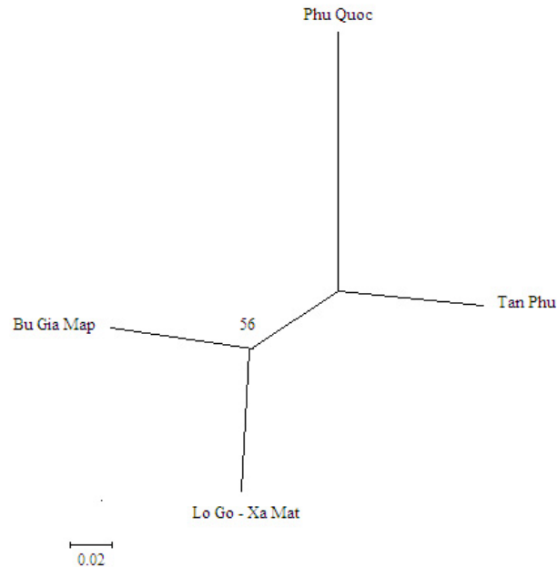
Figure 1. Neighbor joining tree of 4 populations based on Nei's chord distance.
