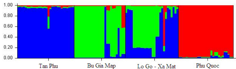
Figure 2. Bar plot of admixture assignment for four populations to the clusters ( K = 3 ) based on Bayesian analysis.
