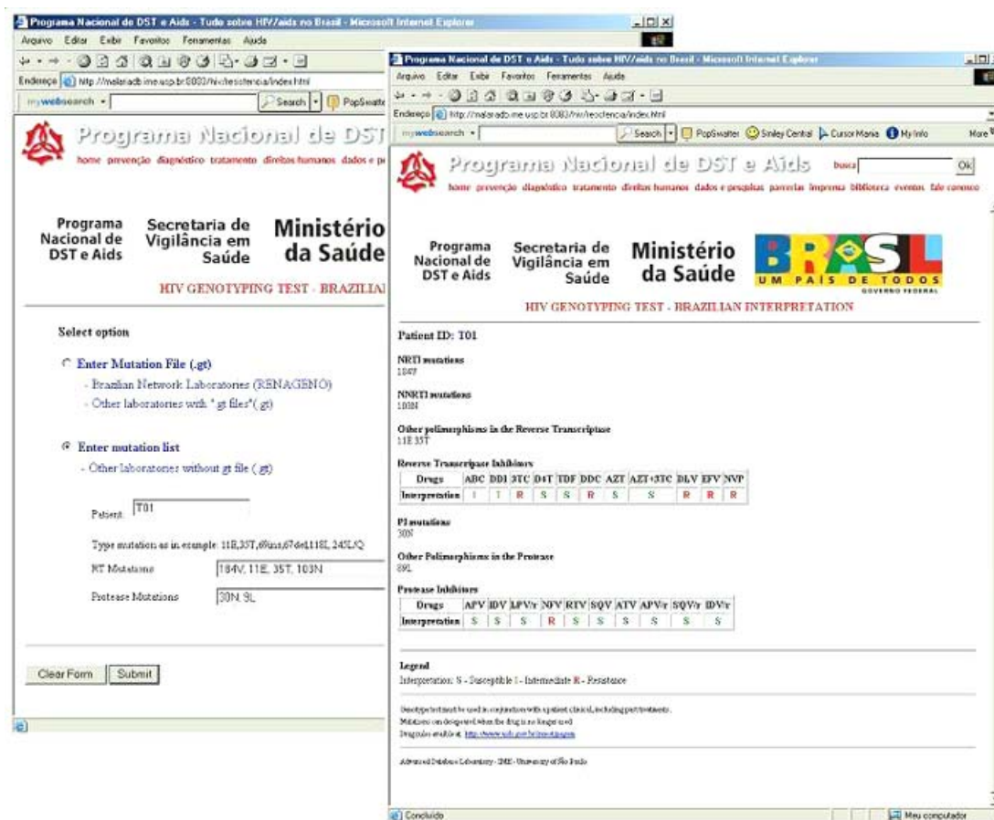
Figure 5. HIV drug resistance interpretation tool integrated into DBCollHIV.
