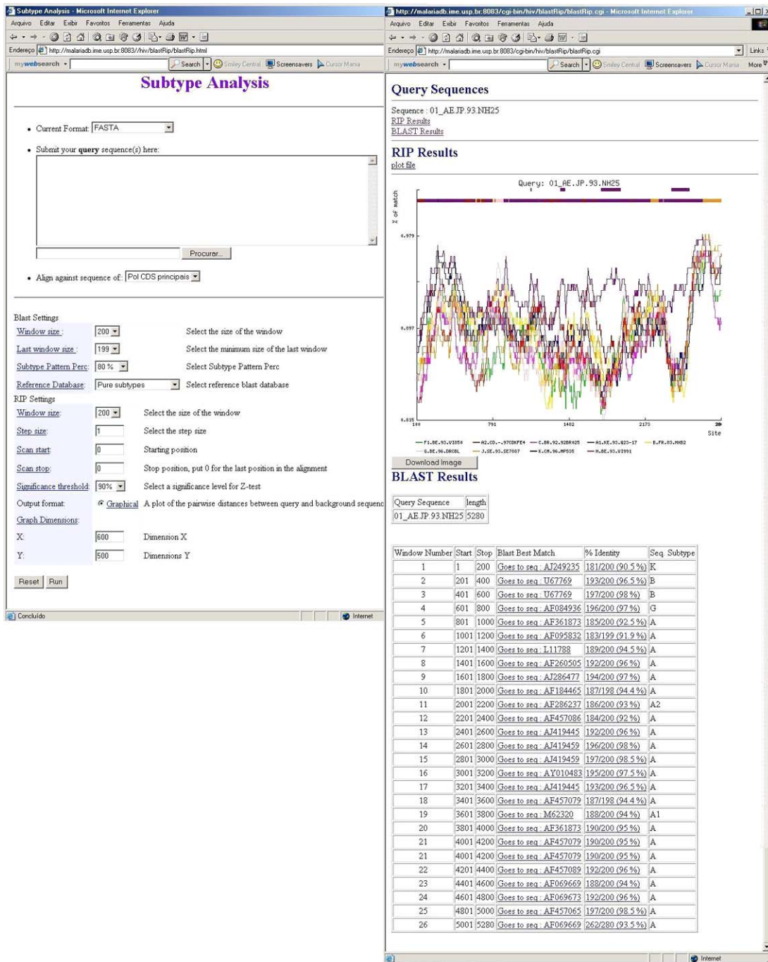
Figure 7. HIV subtype tool integrated into DBCollHIV.
