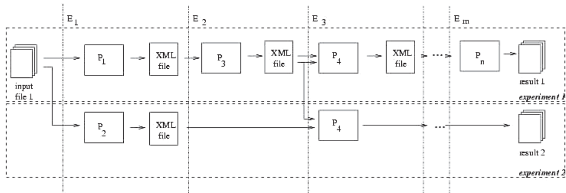
Figure 1. Scheme of integration used by DBCollHIV.
