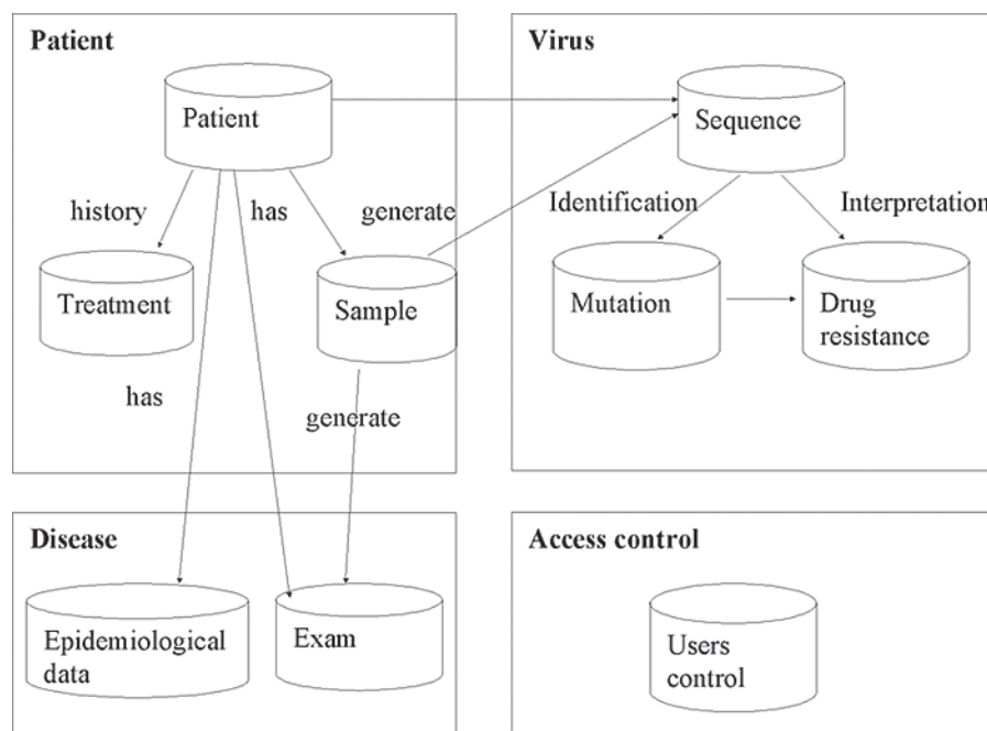
Figure 2. Modules of HIV DBCollHIV and their interactions.
